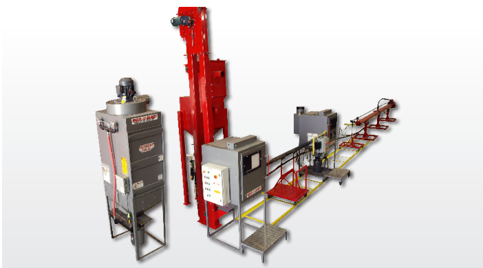
Custom ID pipe blasting system w/ spin blast lance system, floor mounted track assembly, and mechanical recovery system
