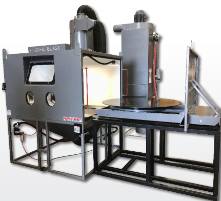
Custom (60"W x 60"D x 40"H) pressure cabinet with H.D. turntable built on door
