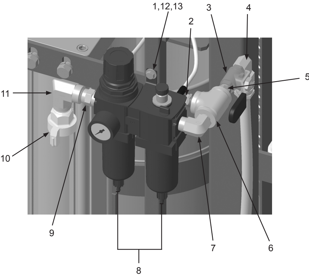
Figure 2: Filter/Lubricator Assembly
