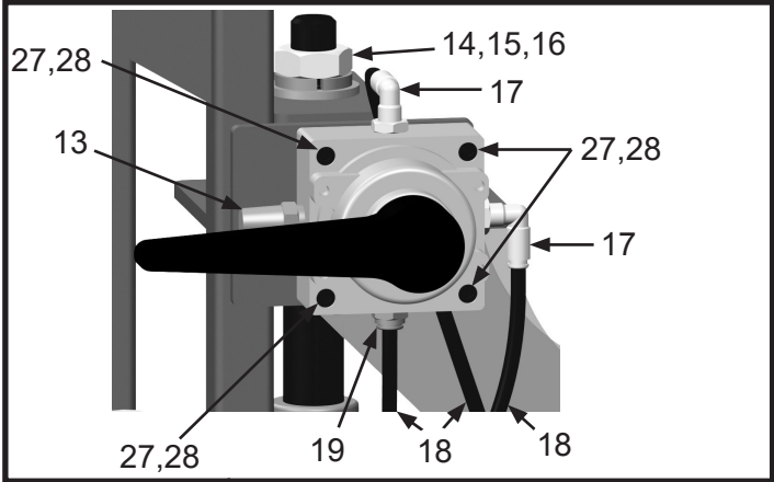
Figure 1: Marco® Elevator Agitator – 5 Gallon (20 Liter) Container
