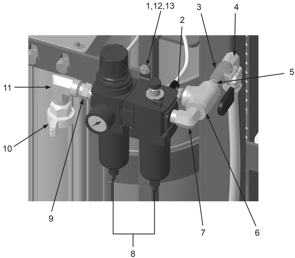
Figure 2: Filter/Lubricator Assembly
