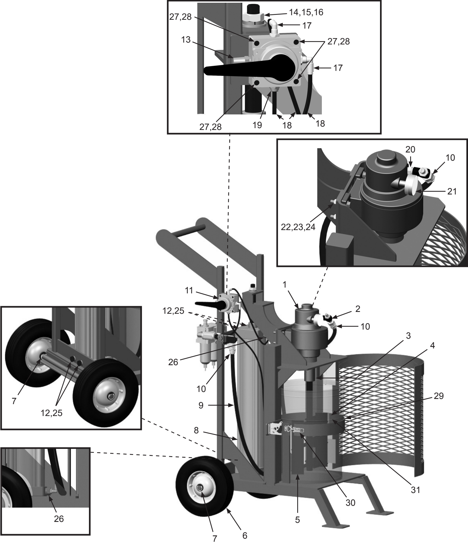
Figure 1: Marco® Elevator Agitator – 5 Gallon (20 Liter) Container
