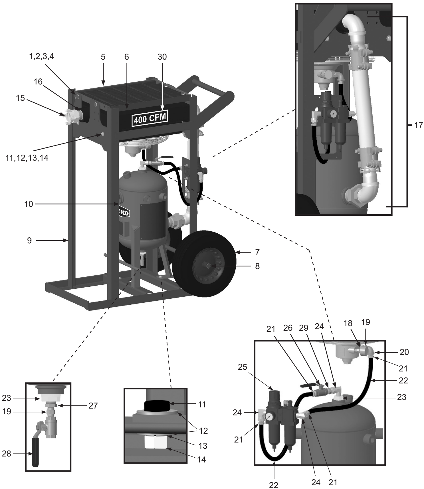
Figure 1: Marco® 400 CFM Cart Mounted Aftercooler With Moisture Separator—Pneumatic
