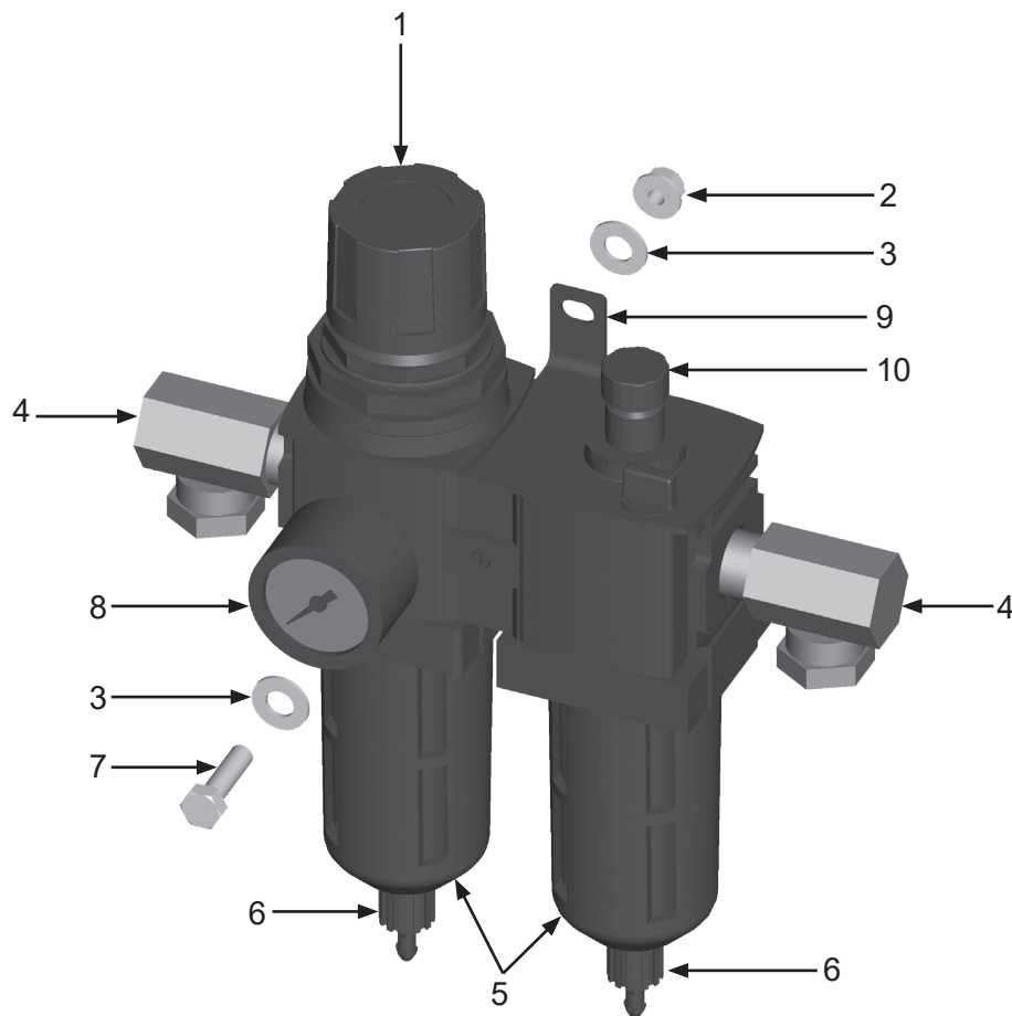
Figure 3: Air Regulator/Lubricator
