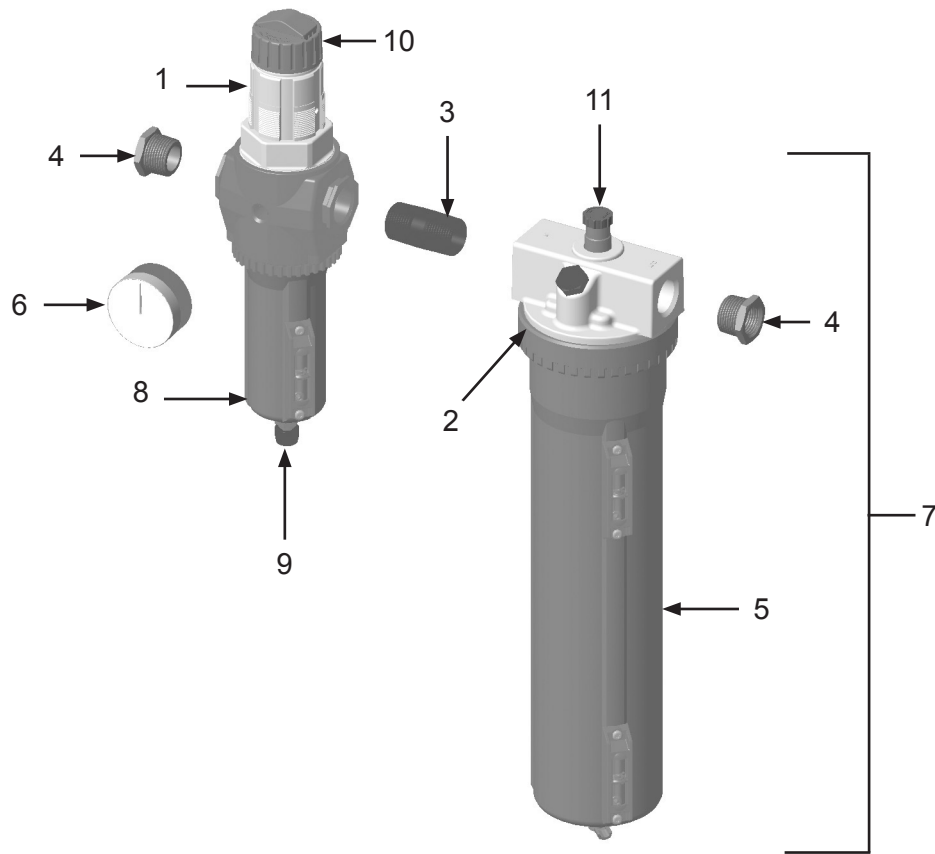
Figure 7: Air Filter/Regulator/Lubricator
