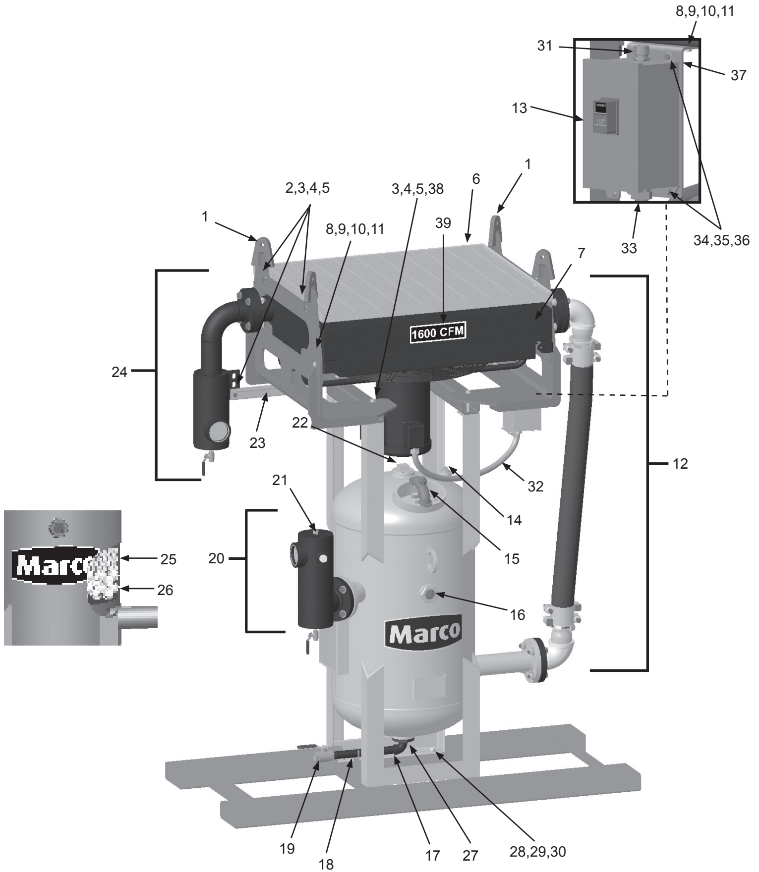
Figure 2: Marco® 1600 CFM Air Dryer—Electric
