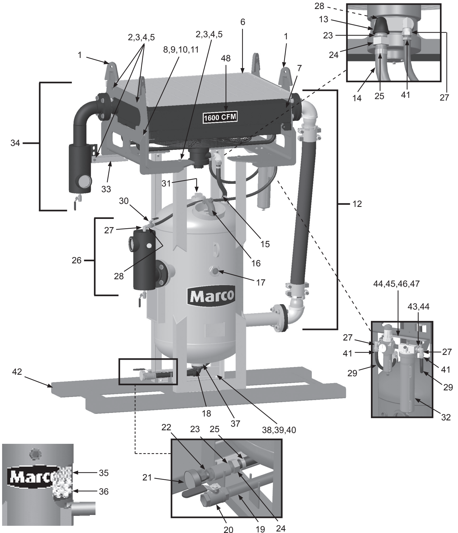
Figure 1: Marco® 1600 CFM Air Dryer—Pneumatic
