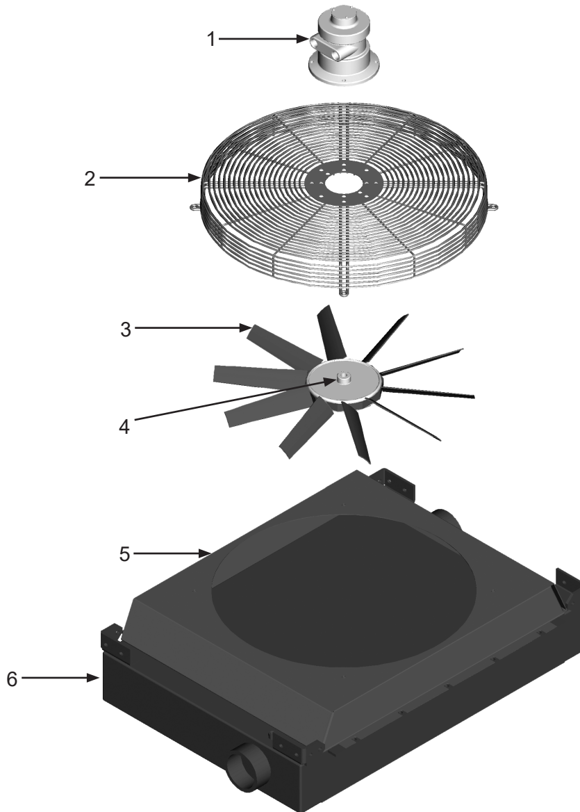
Figure 3: Aftercooler Assembly—Pneumatic
