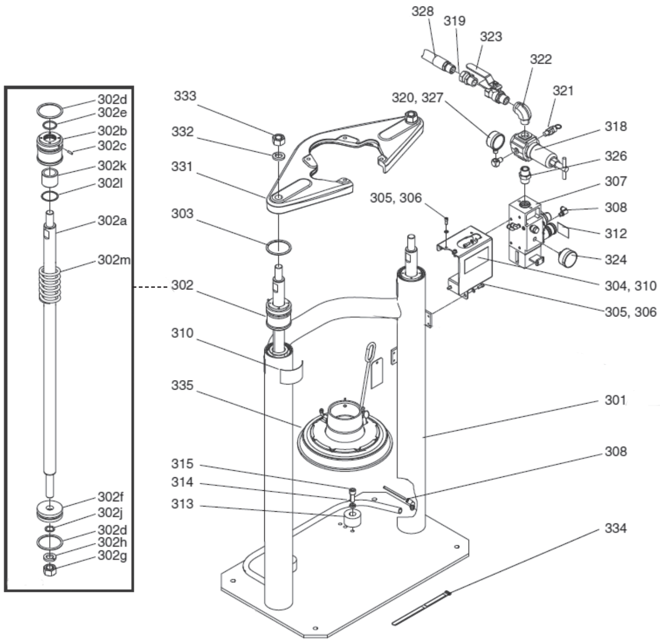
Figure 4: Ram Frame
