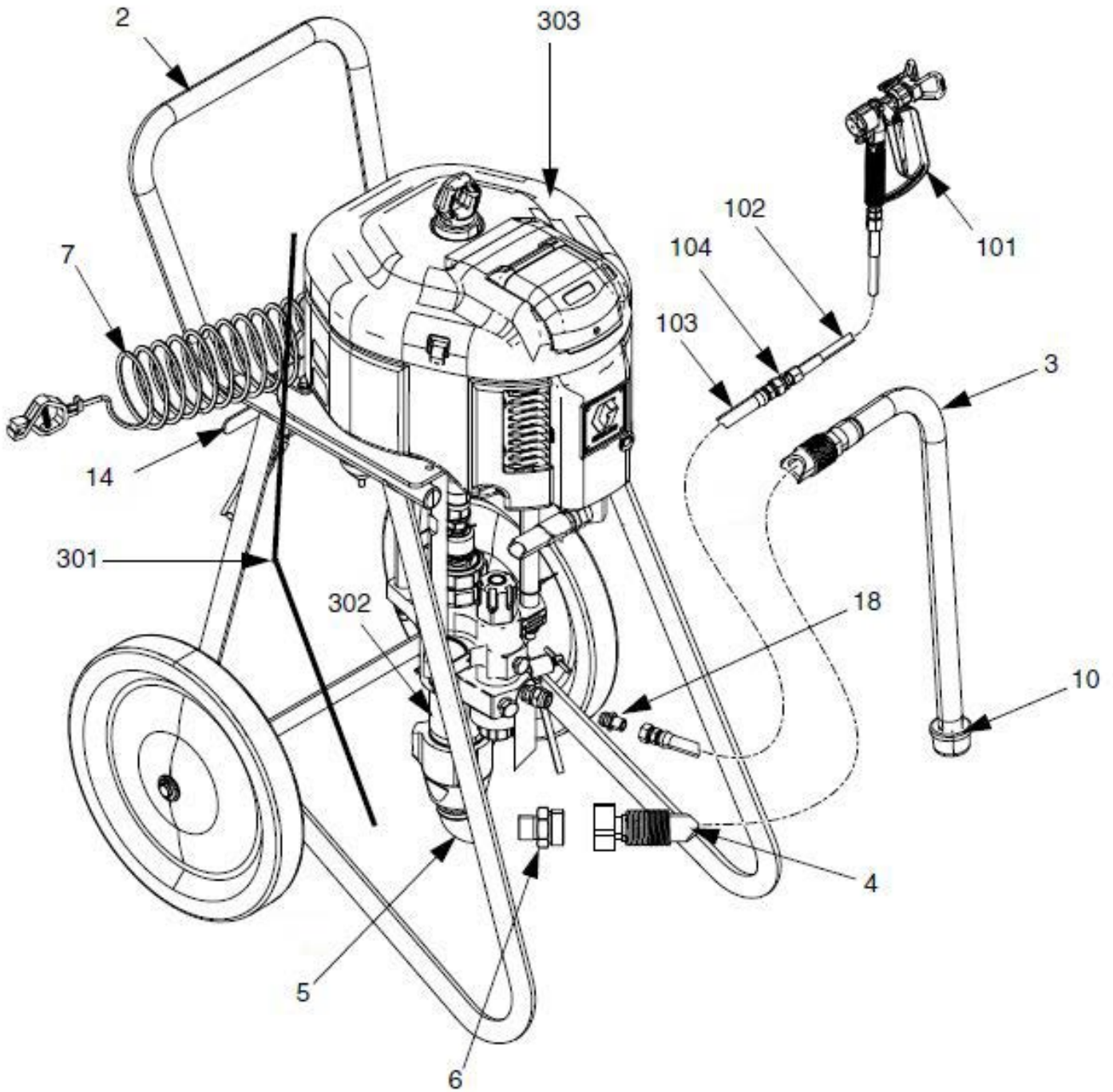
Figure 1: Graco® Xtreme® 60:1 Airless Spray Pumps
