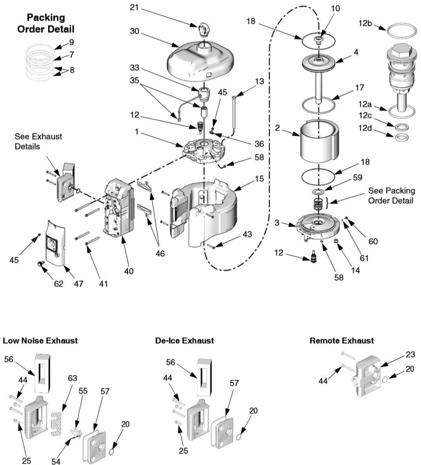
Figure 5: NXT® Model 6500 Air Motor and Exhaust
