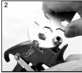
2. Loosen Housing (10).
