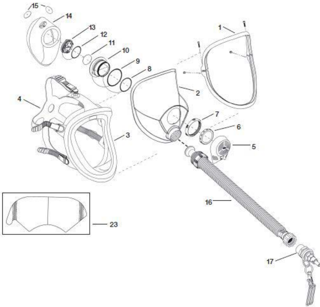
Figure 1: Spectrum Airline Respirator
