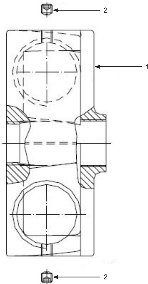
Figure 4: 2" Tornado Large Rotating Head Assembly
