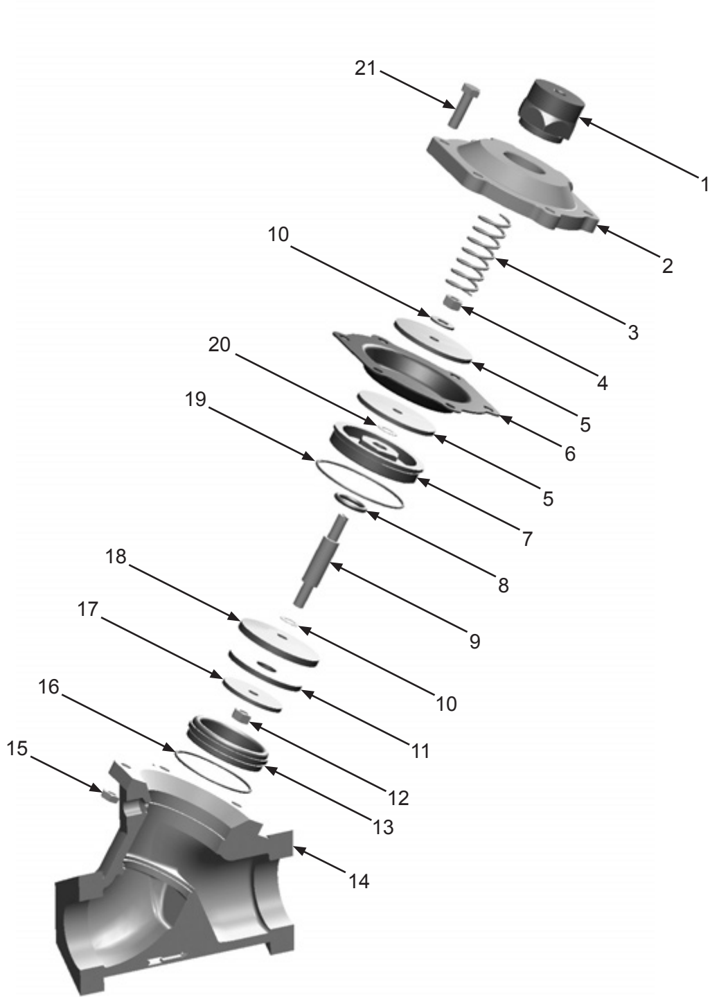
Figure 4: Blastmaster® 2" GateKeeper Air Valve
