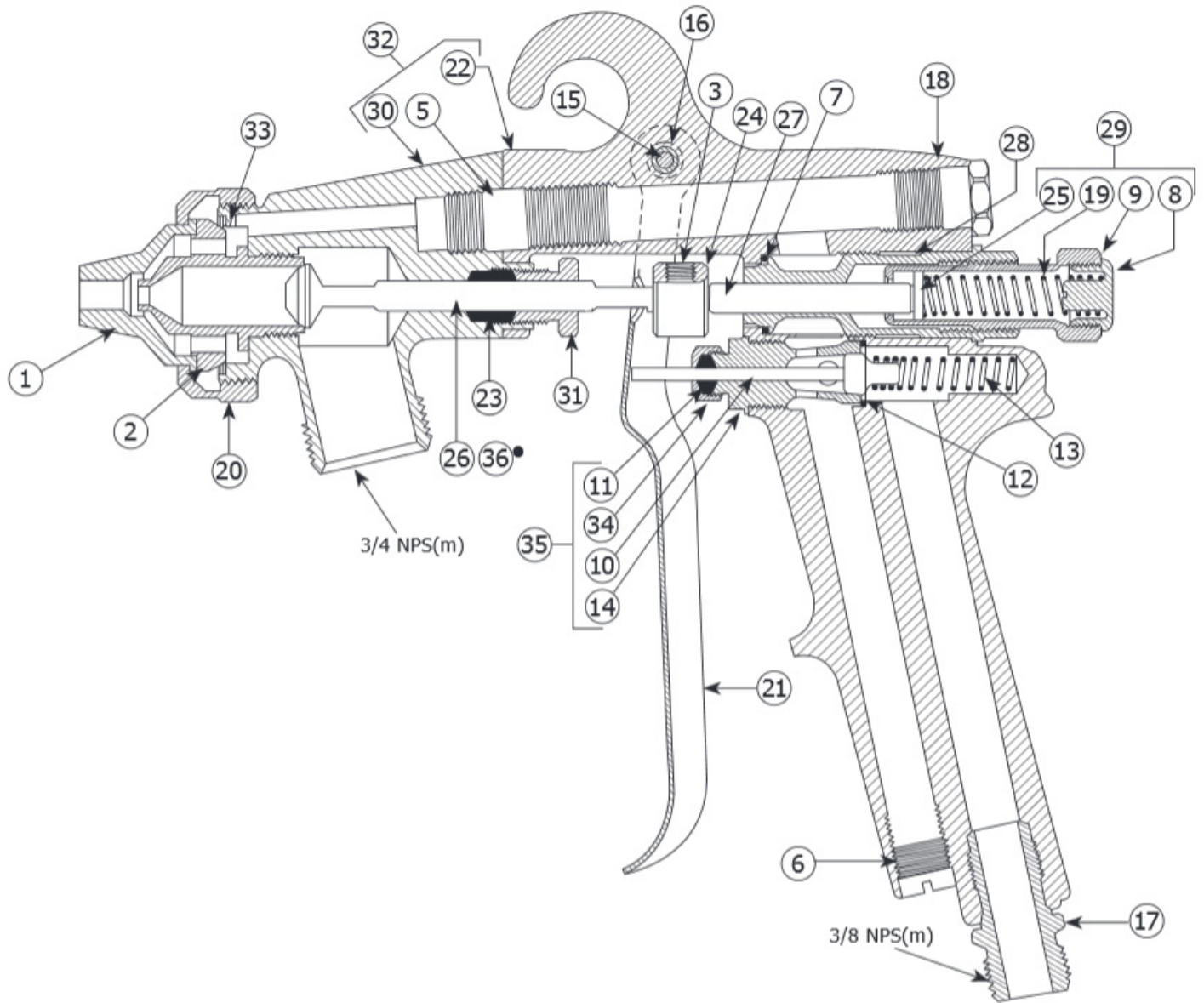
Figure 1: Binks® 7E2 Air Spray Gun
