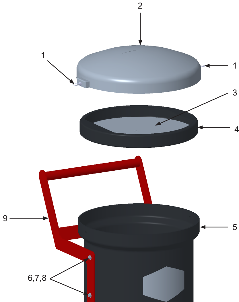
Figure 1: Lid, Screen, & Frame
